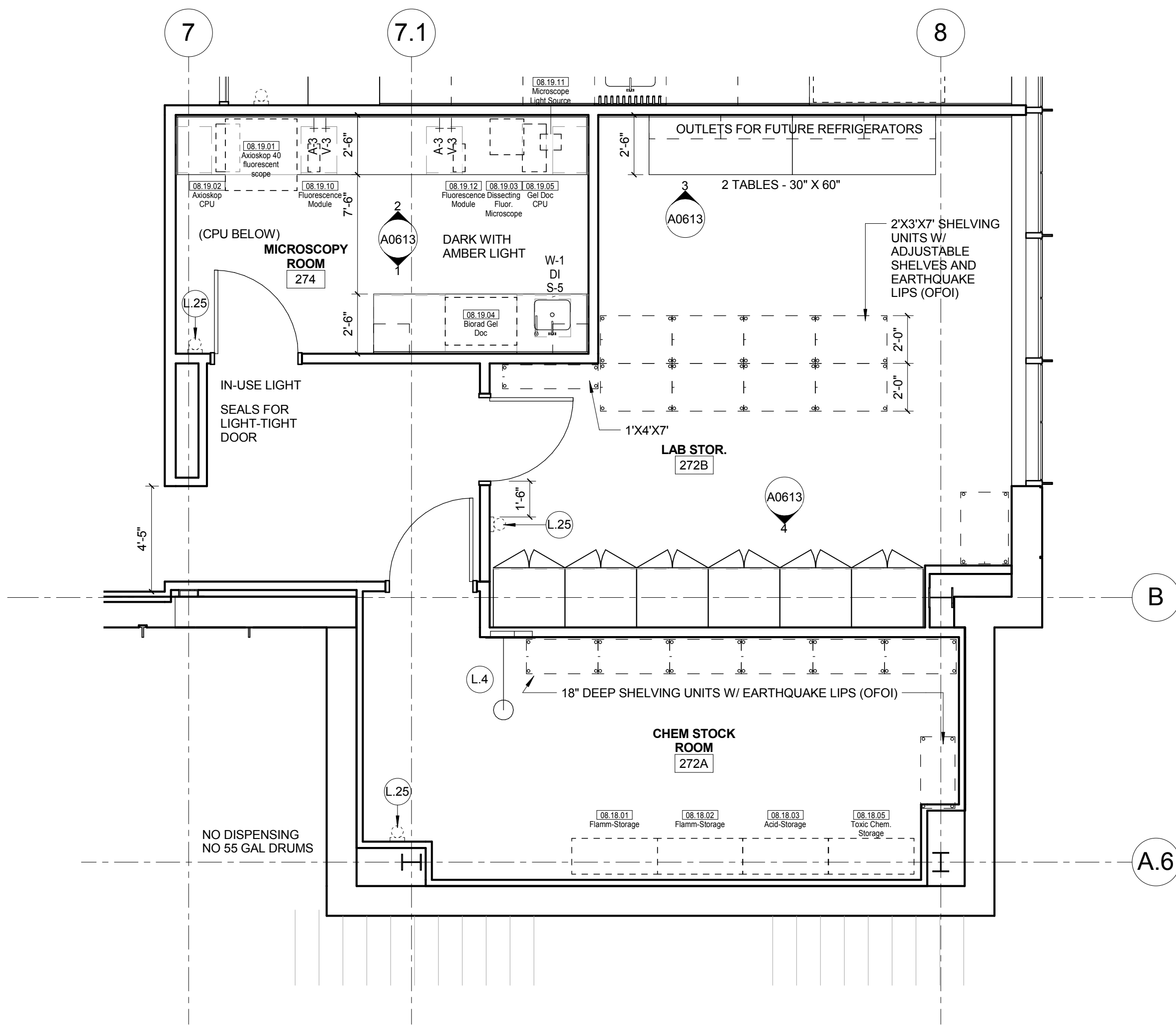
2 LEVEL 02 - AREA A - EAST - SOUTH END 1/4" = 1'-0"
